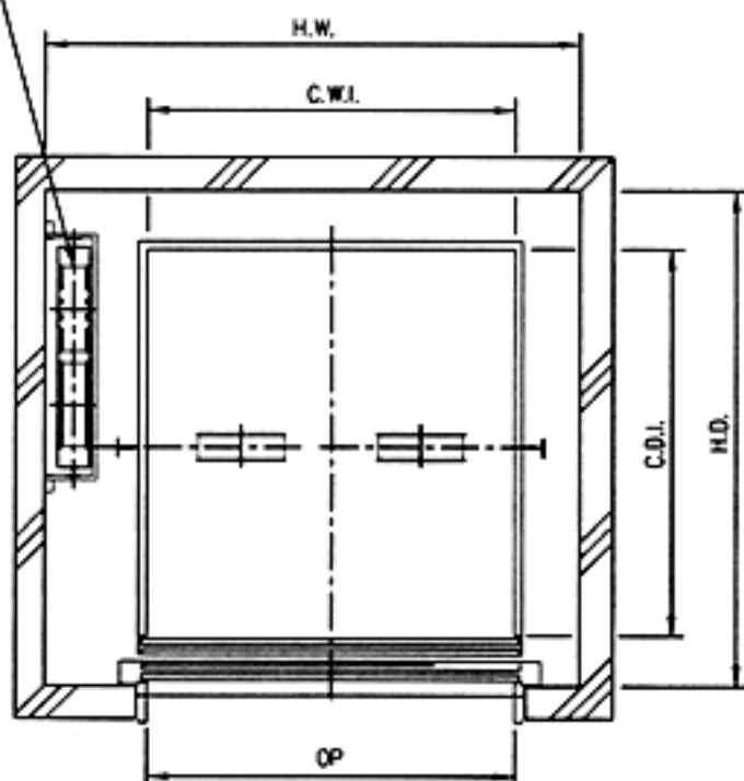
HOISTWAY PLAN
